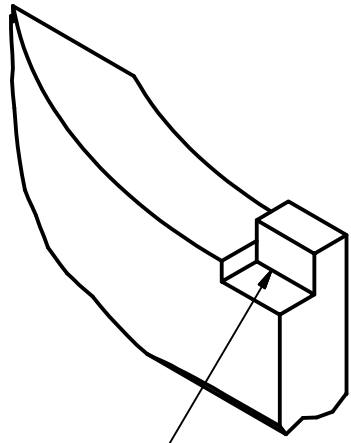
DETAIL OF DOG LEG JOINT
