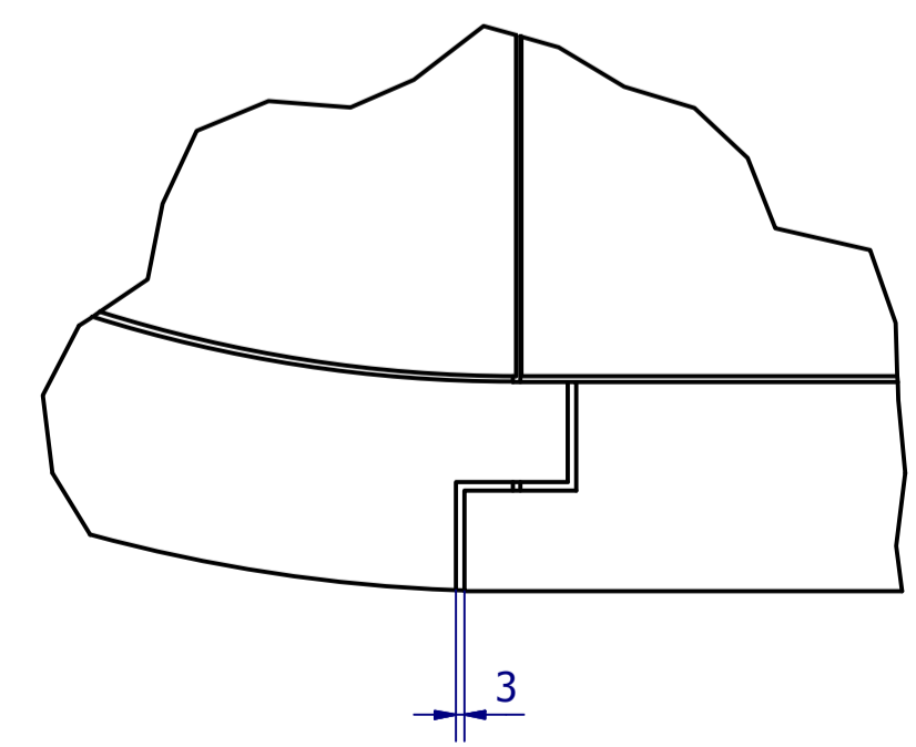
B (1:3) DETAIL OF DOG LEG JOINT
