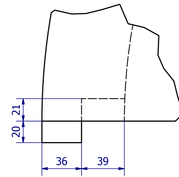
G ( 1 : 2 ) DETAIL OF DOG LEG JOINT
